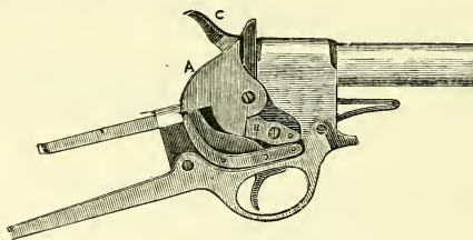
Mechanism of the Remington Rifle.
